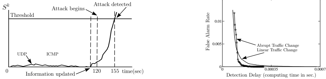
Figure 1: Left: An illustration of sequential change–point detection. Here one particular run of a simulated UDP DoS attack is shown. Right: A summary of the relationship between the detection delay and the false alarm rate for simulated SYN DoS attack. The detection delay is measured using the CPU time used by the detection algorithm.
